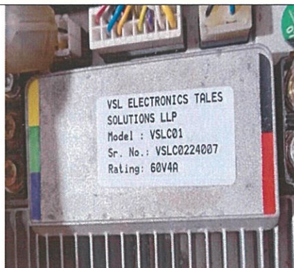
7. DO DRIVE Controller
